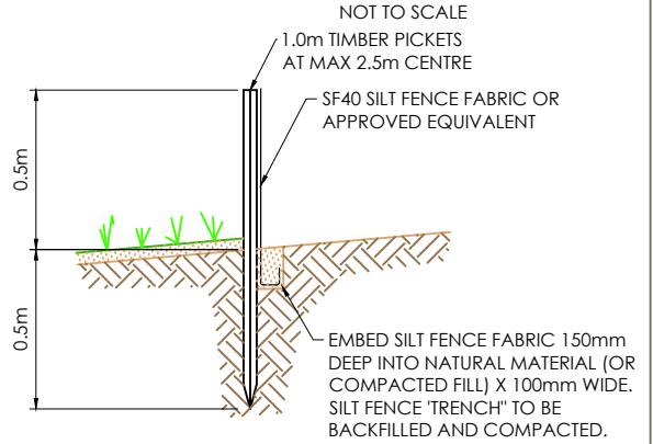
SILT FENCE (SF) NOT TO SCALE
