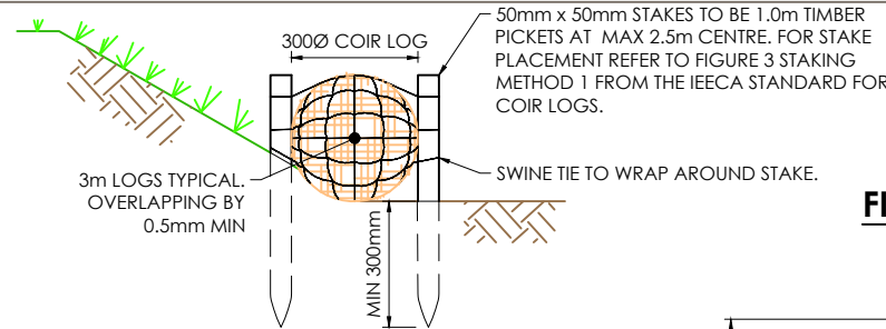
COIR LOG (TYPICAL PLACEMENT) GENERALLY IN ACCORDANCE WITH IEECA GUIDELINES. SCALE 1:20
