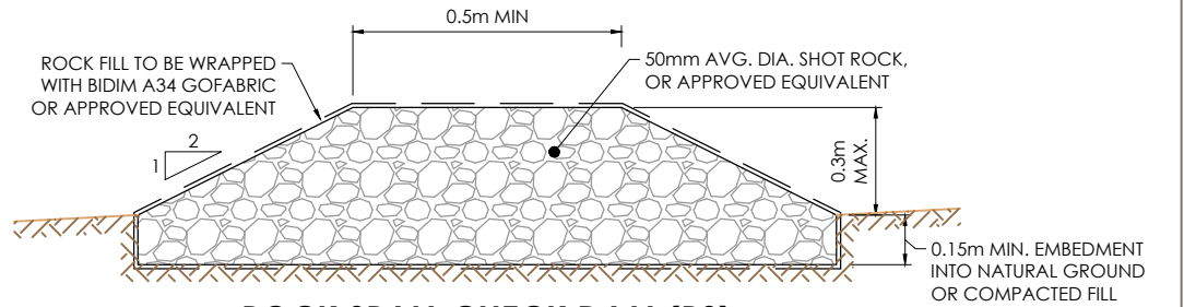
ROCK SPALL CHECK DAM (RS) NOT TO SCALE
